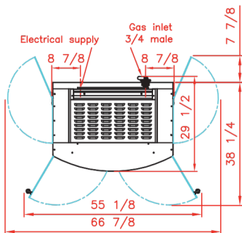
Top view Rotisserie with roof
