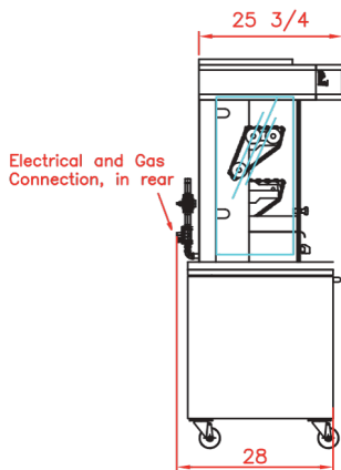
Side view Rotisserie with roof
