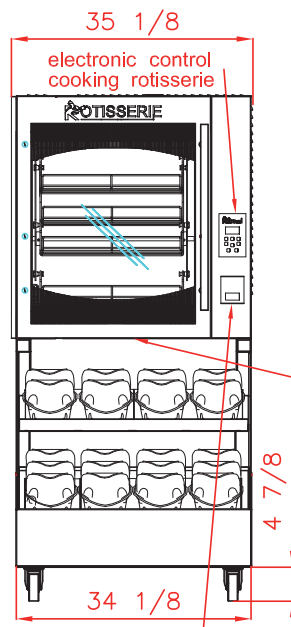
Front view client side Top view
