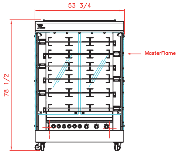
Front view Rotisserie with roof
