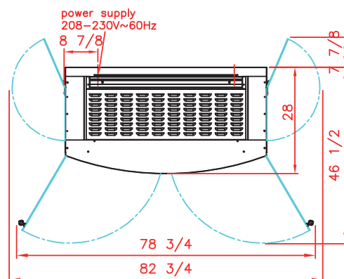
Top view Rotisserie with roof
