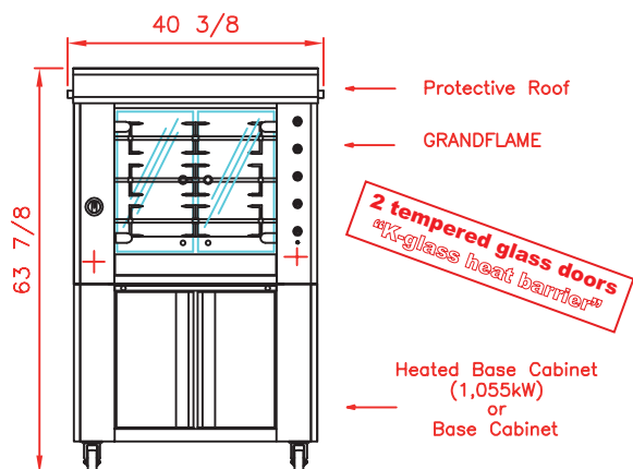
Front view Rotisserie with roof
