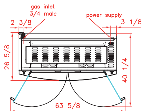
Top view Rotisserie with roof
